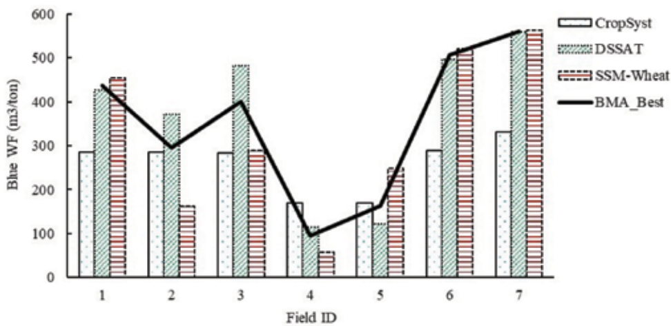
Fig. 5. Comparison of blue WF calculated by individual crop models and BMA
